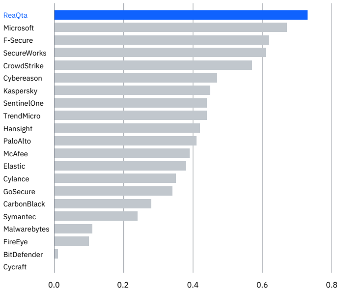
Attack coverage per alert generated (signal-to-noise ratio)
